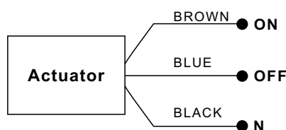
Three-Wire two-Control Valve
